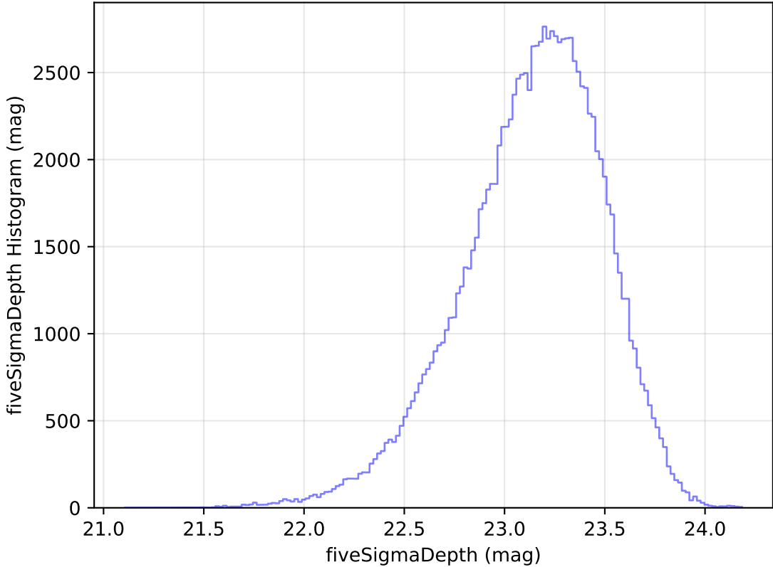
too_elab_heavy_r64_d3_ugrizy_v3.4_10yrs WFD u band: fiveSigmaDepth Histogram
