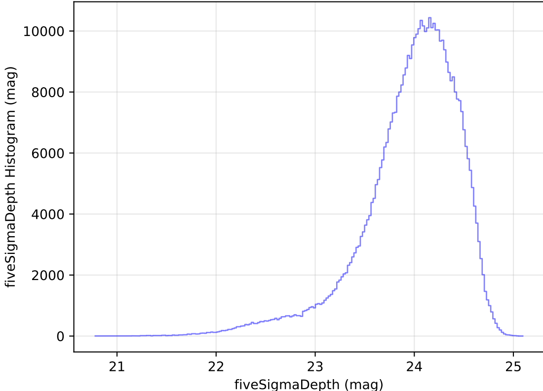
too_elab_heavy_r64_d3_ugrizy_v3.4_10yrs WFD r band: fiveSigmaDepth Histogram
