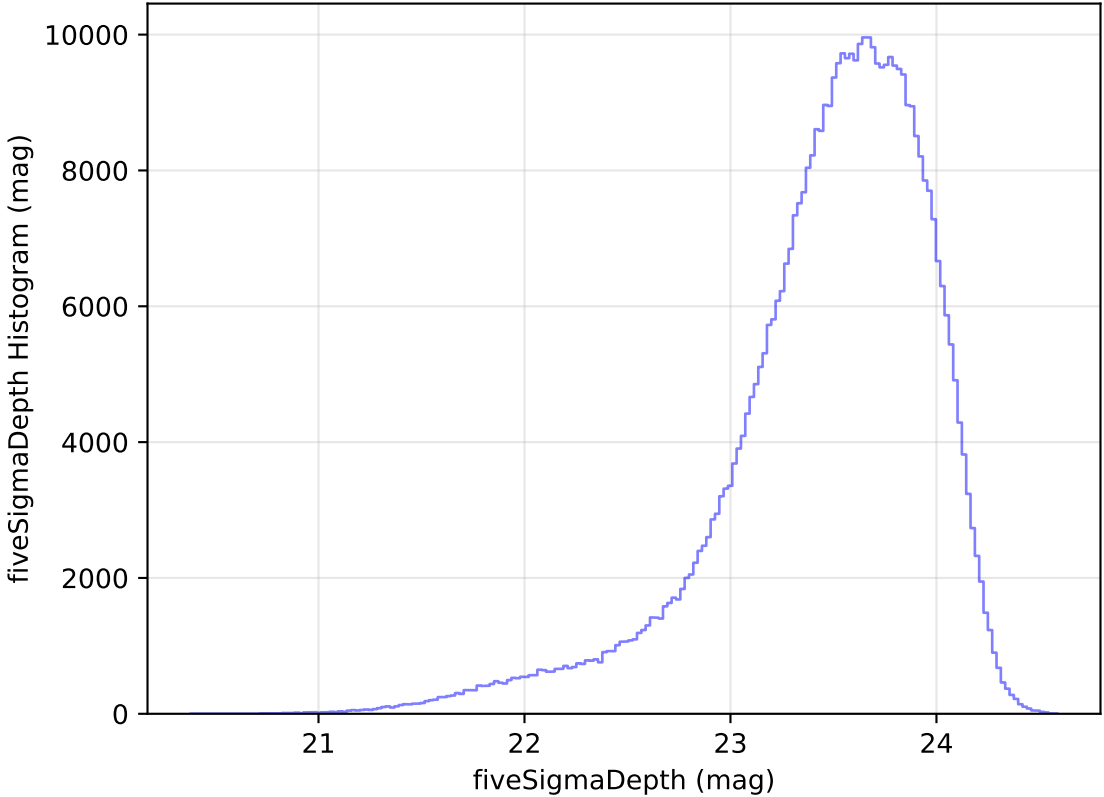
too_elab_heavy_r64_d3_ugrizy_v3.4_10yrs WFD i band: fiveSigmaDepth Histogram
