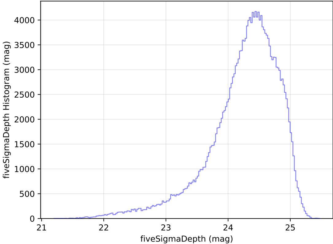
too_elab_heavy_r64_d3_ugrizy_v3.4_10yrs WFD g band: fiveSigmaDepth Histogram
