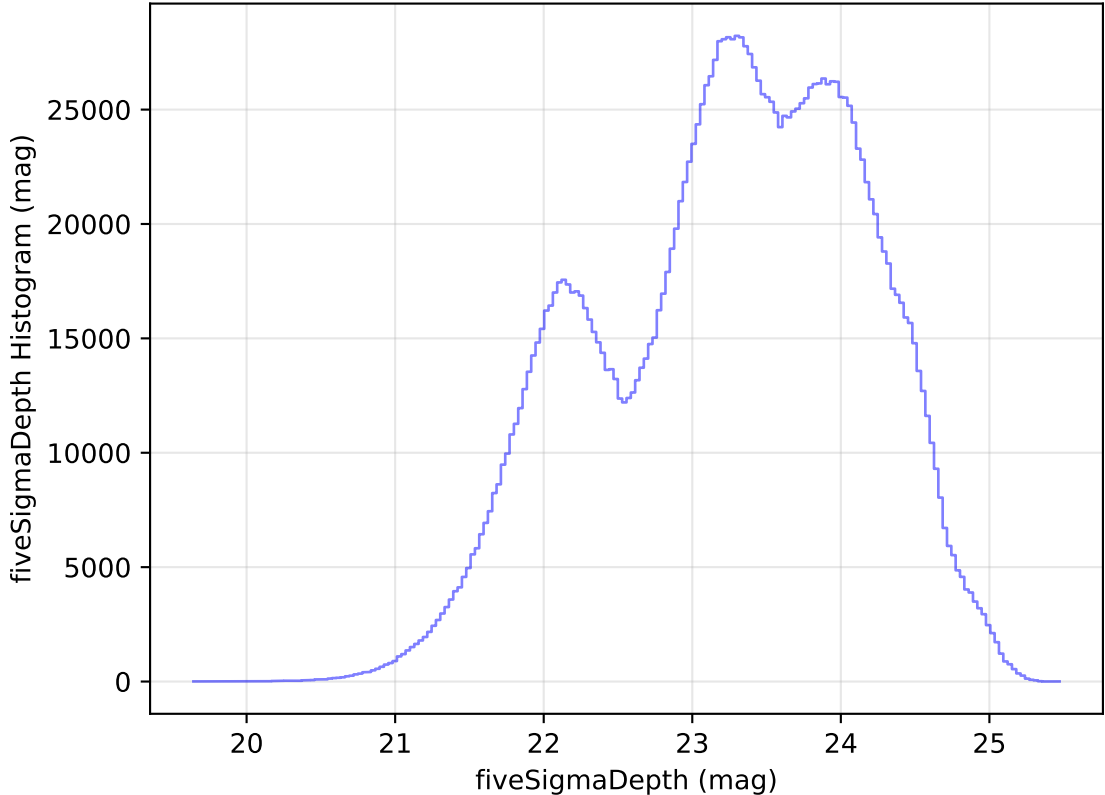
too_elab_heavy_r64_d3_ugrizy_v3.4_10yrs WFD all bands: fiveSigmaDepth Histogram
