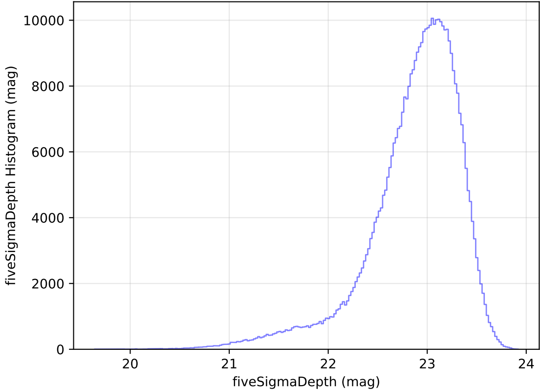
too_elab_heavy_r64_d3_ugrizy_v3.4_10yrs All sky z band: fiveSigmaDepth Histogram
