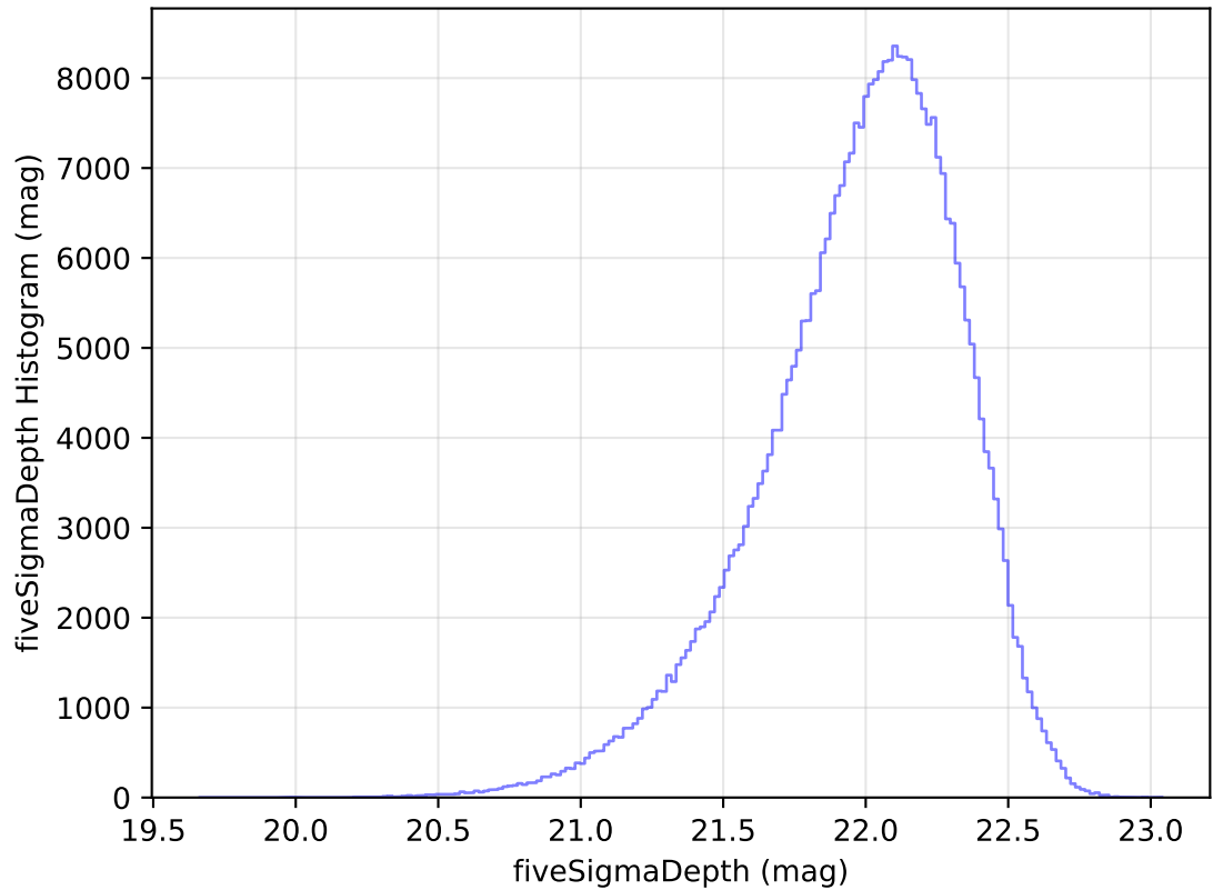
too_elab_heavy_r64_d3_ugrizy_v3.4_10yrs All sky y band: fiveSigmaDepth Histogram
