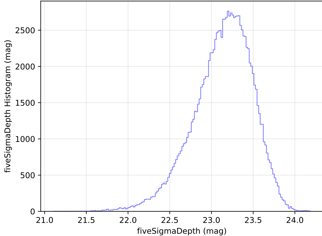
too_elab_heavy_r64_d3_ugrizy_v3.4_10yrs All sky u band: fiveSigmaDepth Histogram
