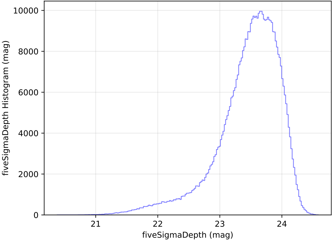
too_elab_heavy_r64_d3_ugrizy_v3.4_10yrs All sky i band: fiveSigmaDepth Histogram
