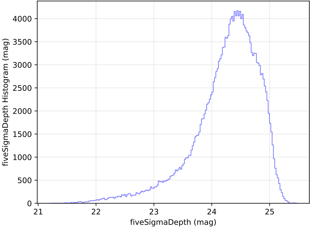
too_elab_heavy_r64_d3_ugrizy_v3.4_10yrs All sky g band: fiveSigmaDepth Histogram
