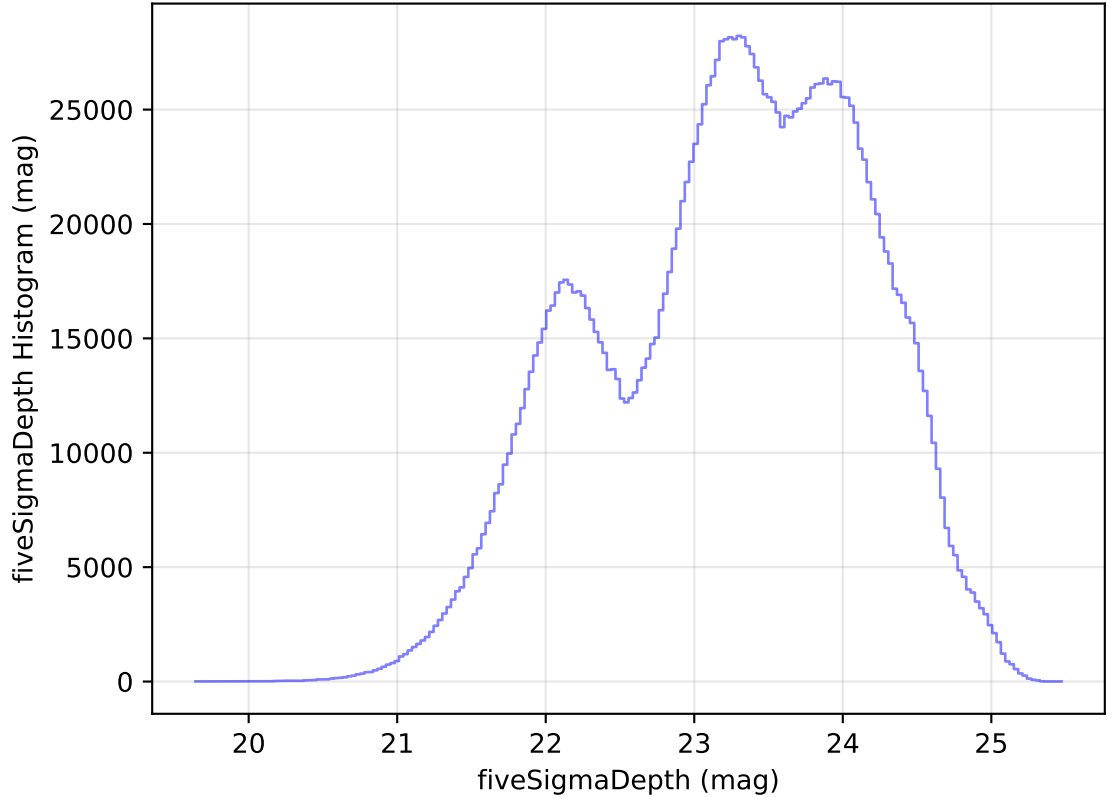
too_elab_heavy_r64_d3_ugrizy_v3.4_10yrs All sky all bands: fiveSigmaDepth Histogram
