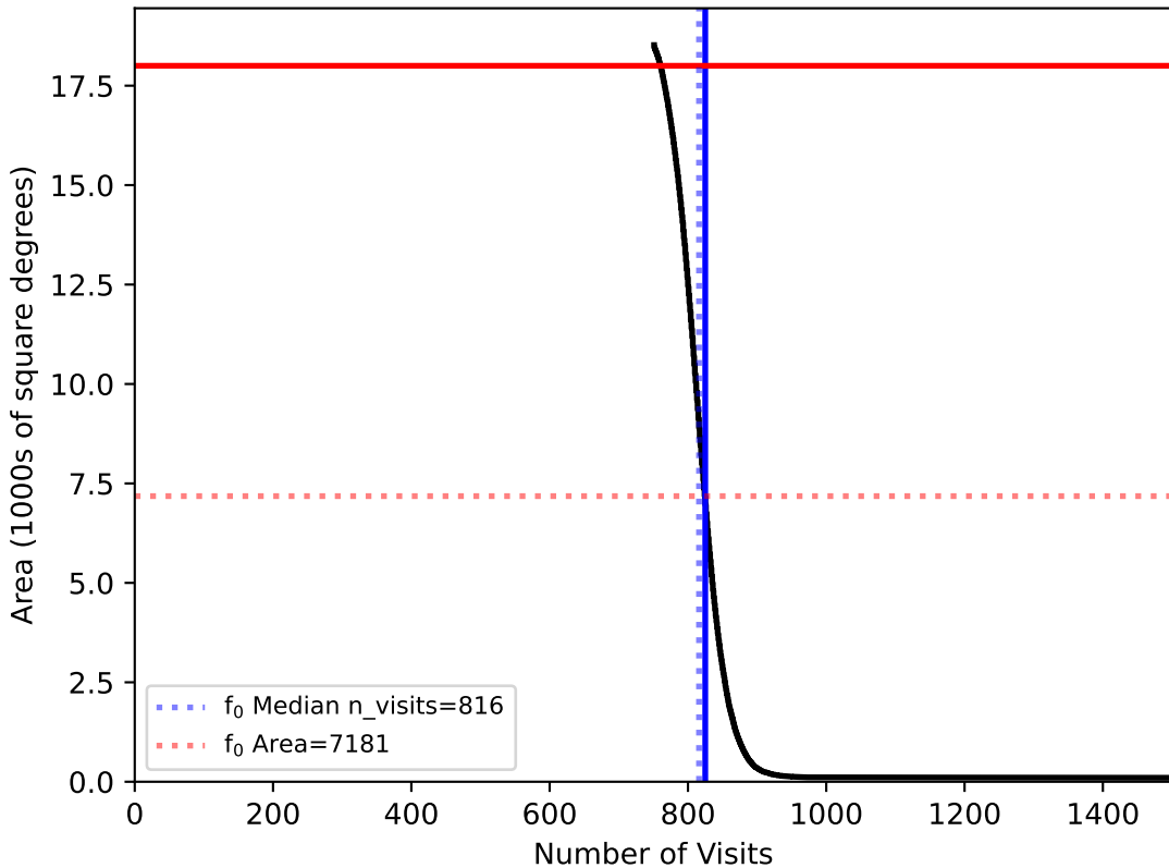
too_elab_heavy_r64_d3_ugrizy_v3.4_10yrs WFD: f0
