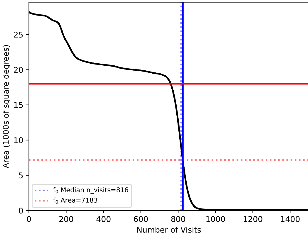
too_elab_heavy_r64_d3_ugrizy_v3.4_10yrs All sky: f0
