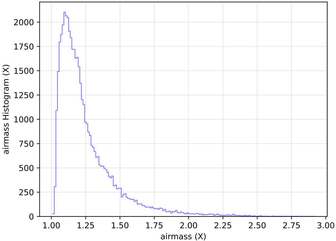
too_elab_heavy_r64_d3_ugrizy_v3.4_10yrs Yr 1 y band: airmass Histogram
