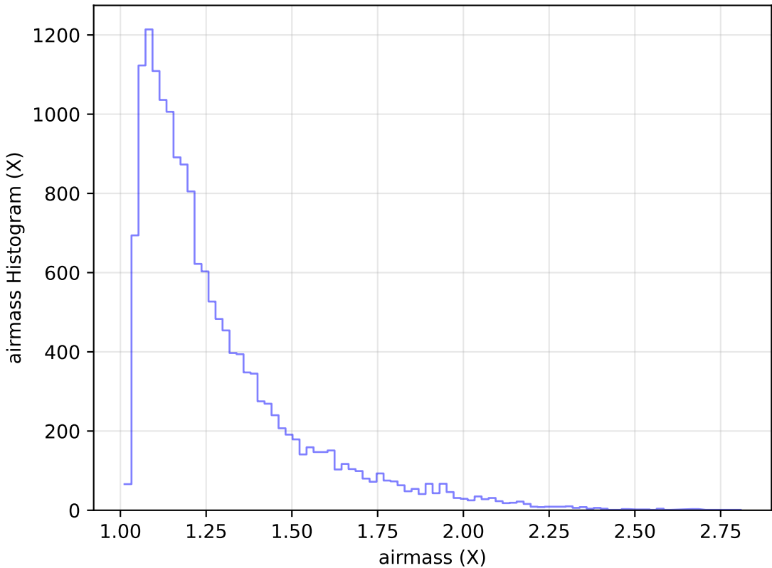
too_elab_heavy_r64_d3_ugrizy_v3.4_10yrs Yr 1 u band: airmass Histogram
