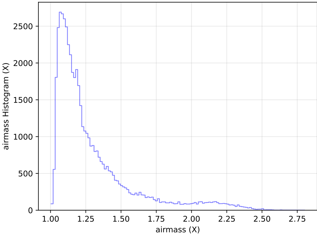
too_elab_heavy_r64_d3_ugrizy_v3.4_10yrs Yr 1 r band: airmass Histogram
