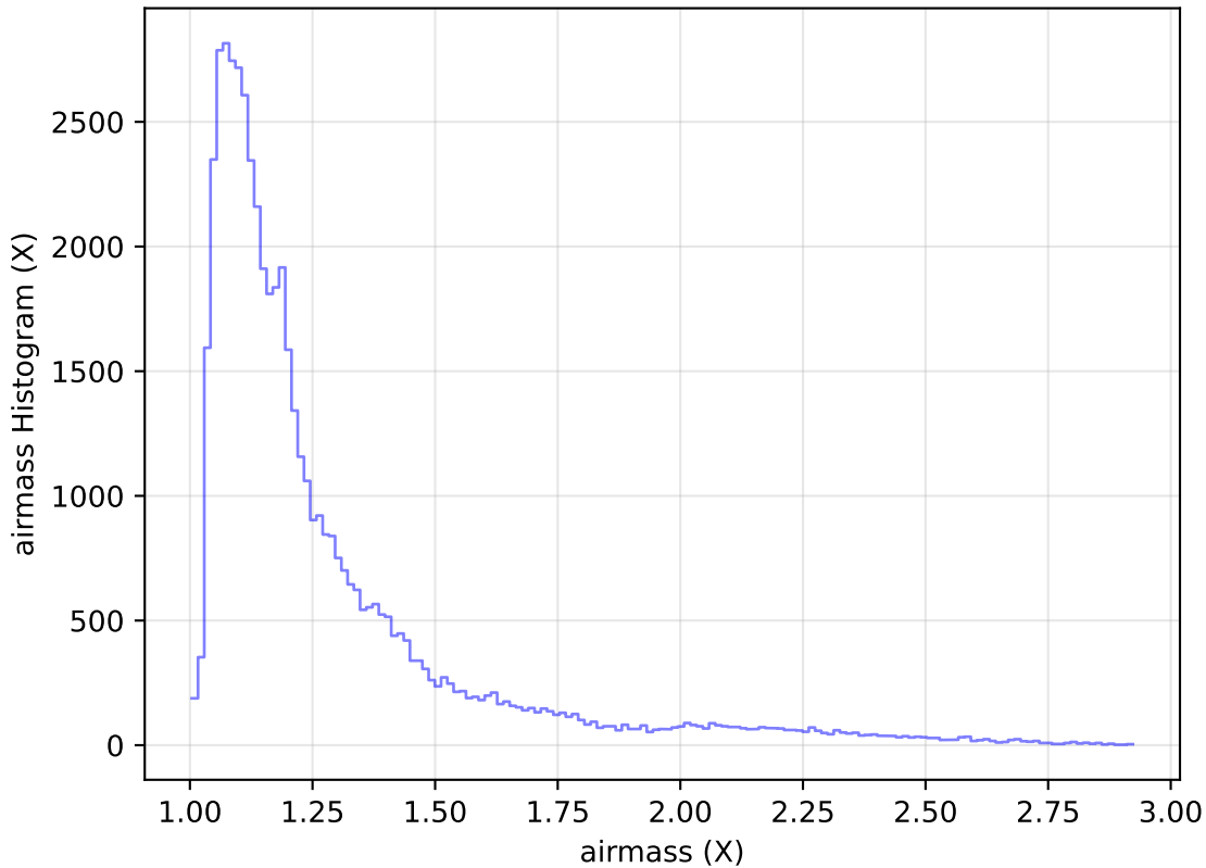
too_elab_heavy_r64_d3_ugrizy_v3.4_10yrs Yr 1 i band: airmass Histogram
