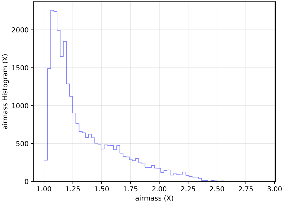
too_elab_heavy_r64_d3_ugrizy_v3.4_10yrs Yr 1 g band: airmass Histogram
