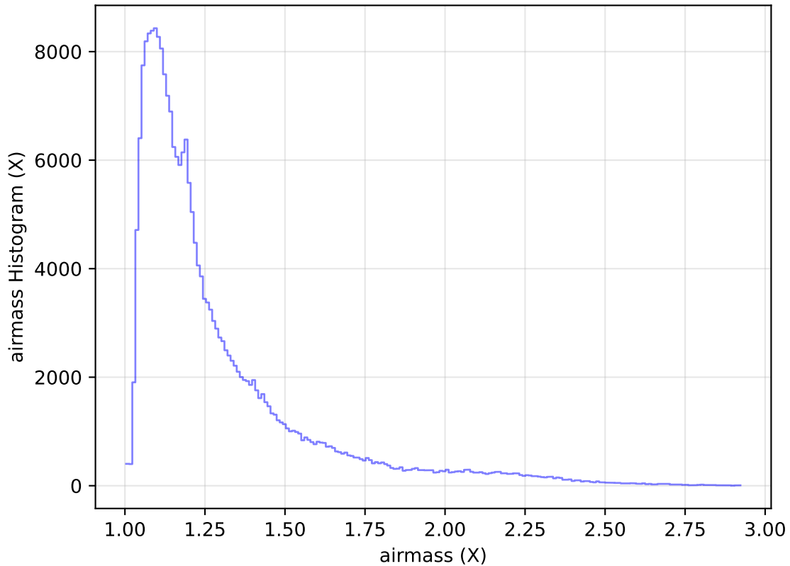
too_elab_heavy_r64_d3_ugrizy_v3.4_10yrs Yr 1 all bands: airmass Histogram
