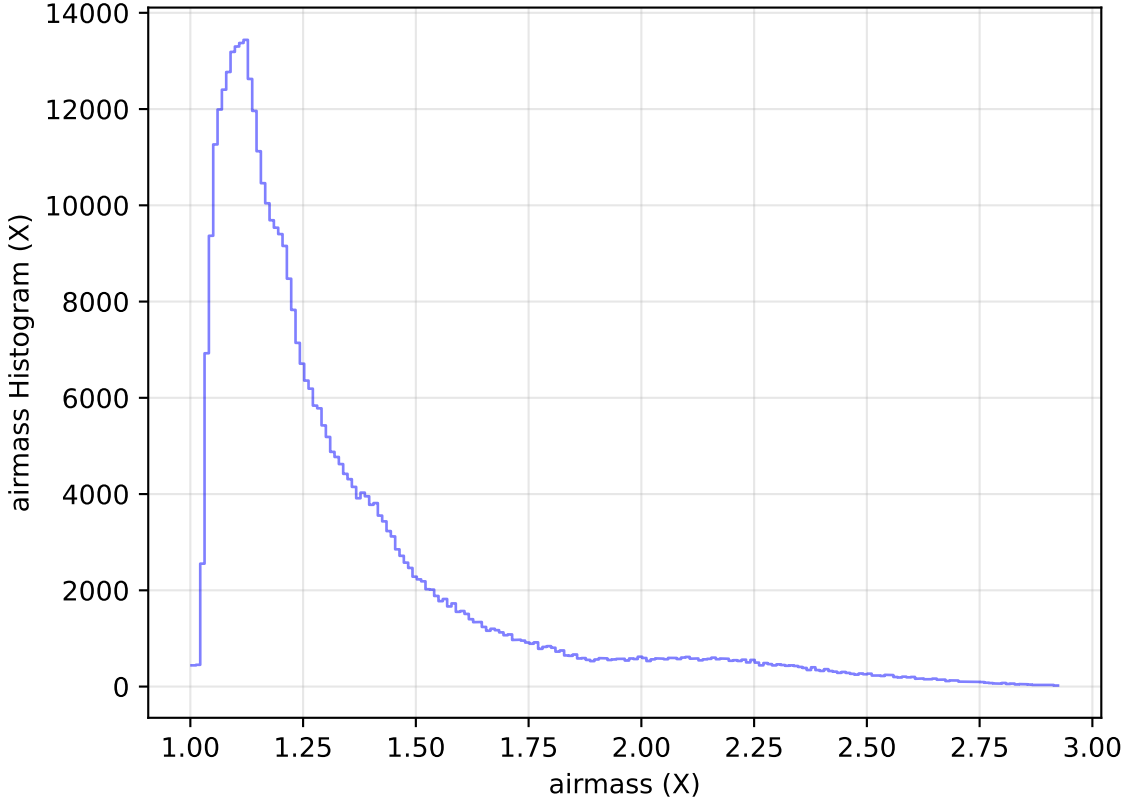
too_elab_heavy_r64_d3_ugrizy_v3.4_10yrs WFD z band: airmass Histogram
