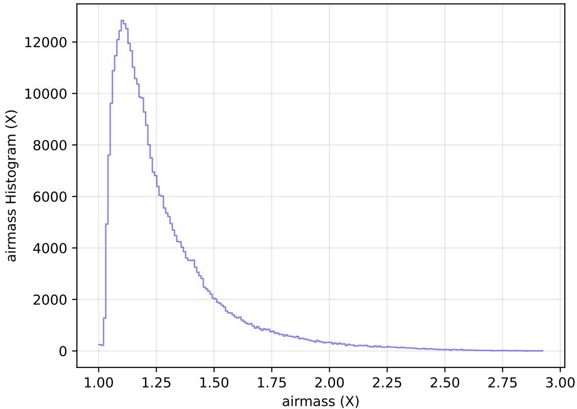
too_elab_heavy_r64_d3_ugrizy_v3.4_10yrs WFD y band: airmass Histogram
