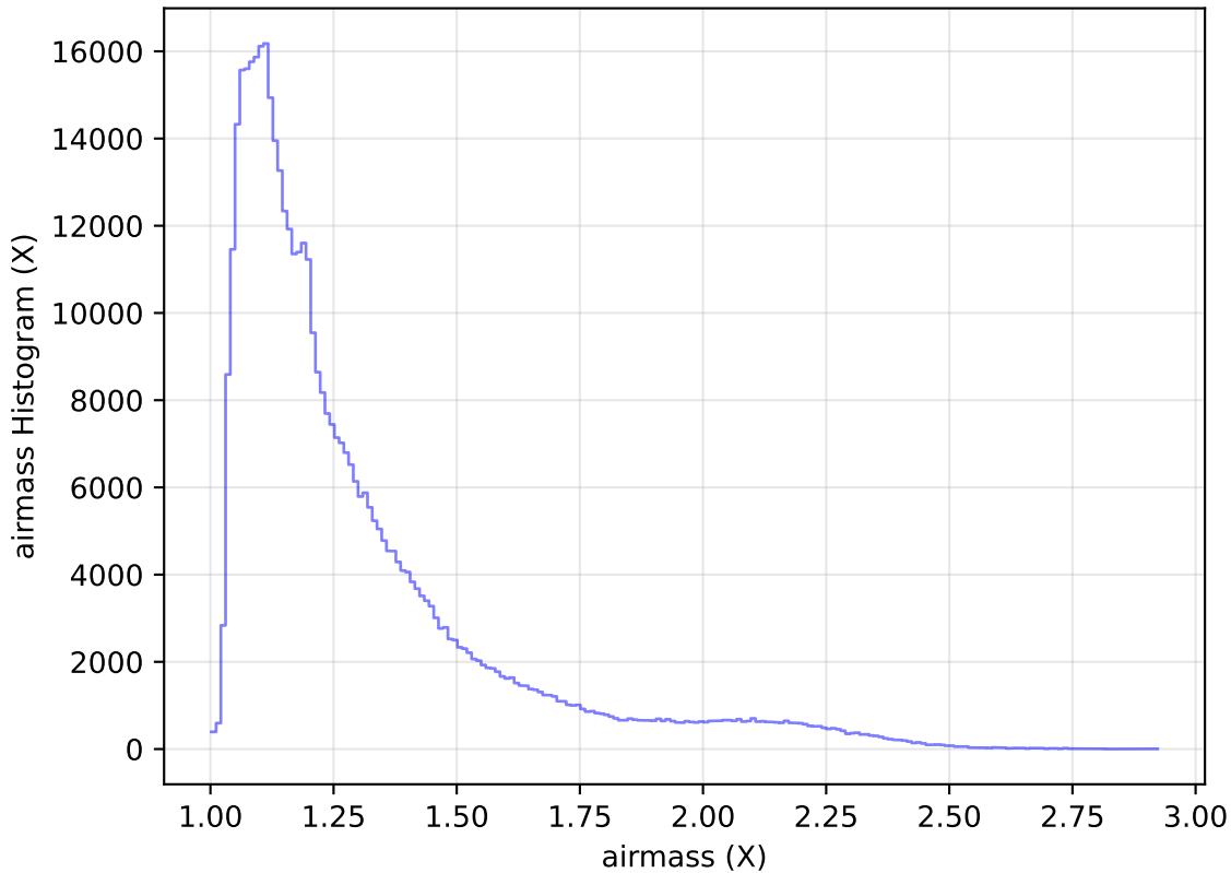
too_elab_heavy_r64_d3_ugrizy_v3.4_10yrs WFD r band: airmass Histogram
