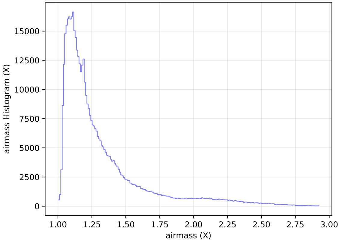
too_elab_heavy_r64_d3_ugrizy_v3.4_10yrs WFD i band: airmass Histogram
