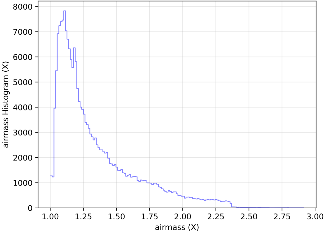
too_elab_heavy_r64_d3_ugrizy_v3.4_10yrs WFD g band: airmass Histogram
