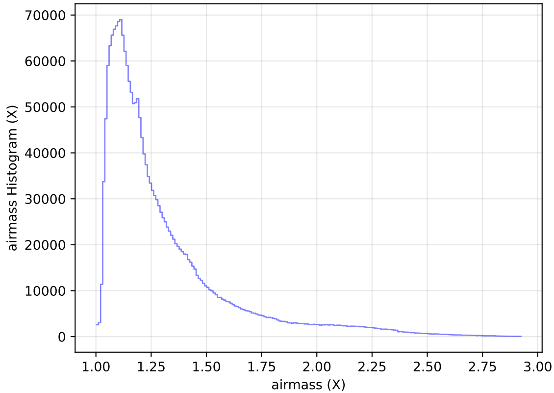
too_elab_heavy_r64_d3_ugrizy_v3.4_10yrs WFD all bands: airmass Histogram
