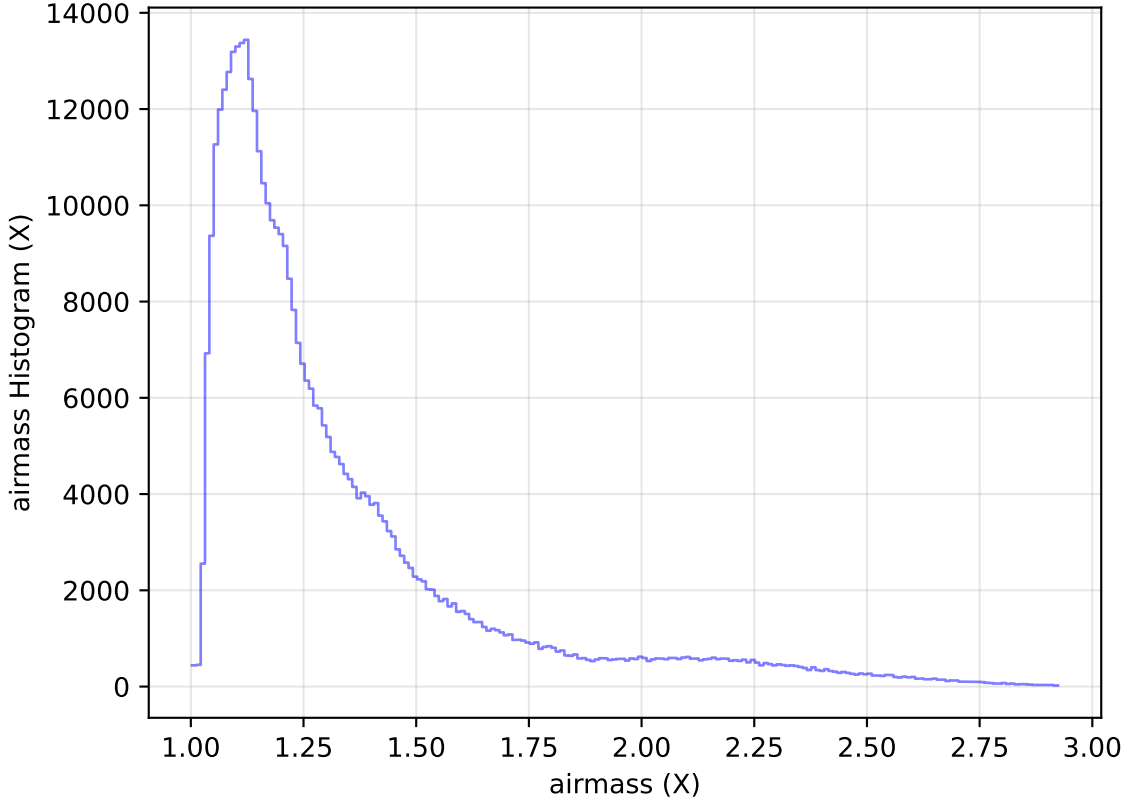
too_elab_heavy_r64_d3_ugrizy_v3.4_10yrs All sky z band: airmass Histogram
