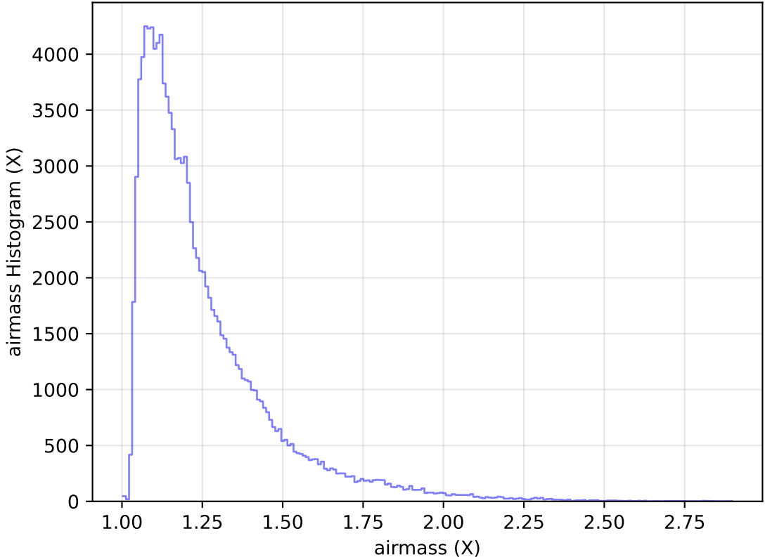
too_elab_heavy_r64_d3_ugrizy_v3.4_10yrs All sky u band: airmass Histogram
