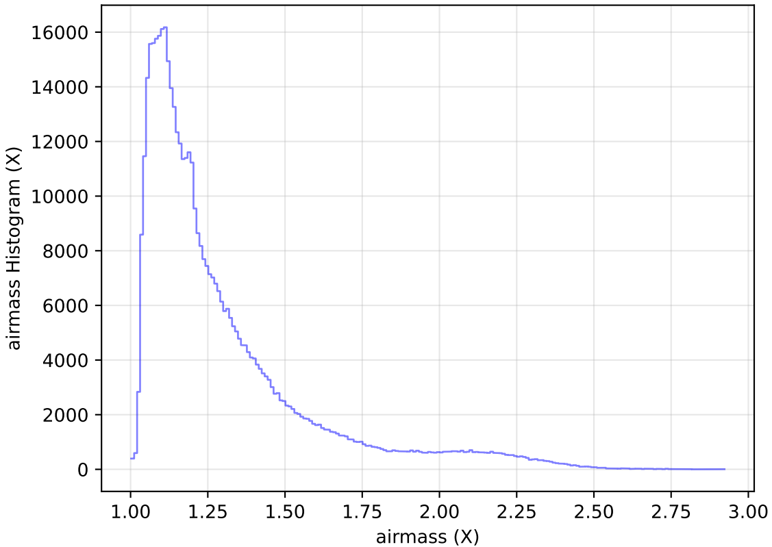
too_elab_heavy_r64_d3_ugrizy_v3.4_10yrs All sky r band: airmass Histogram
