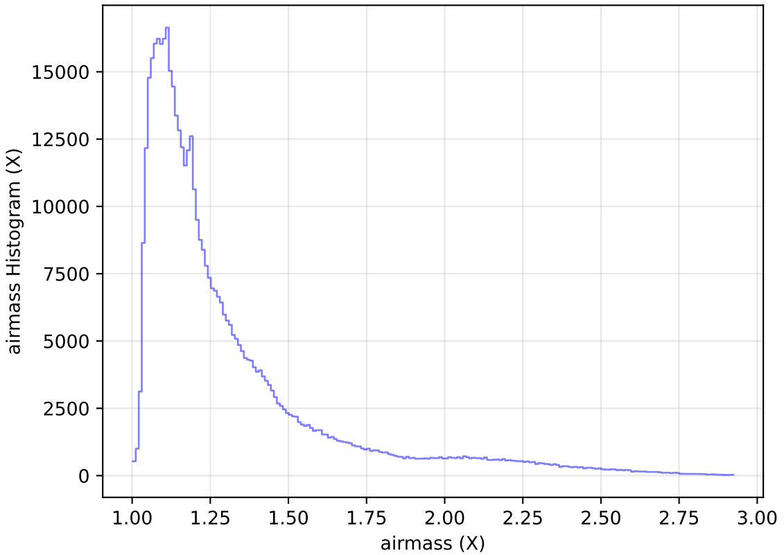
too_elab_heavy_r64_d3_ugrizy_v3.4_10yrs All sky i band: airmass Histogram
