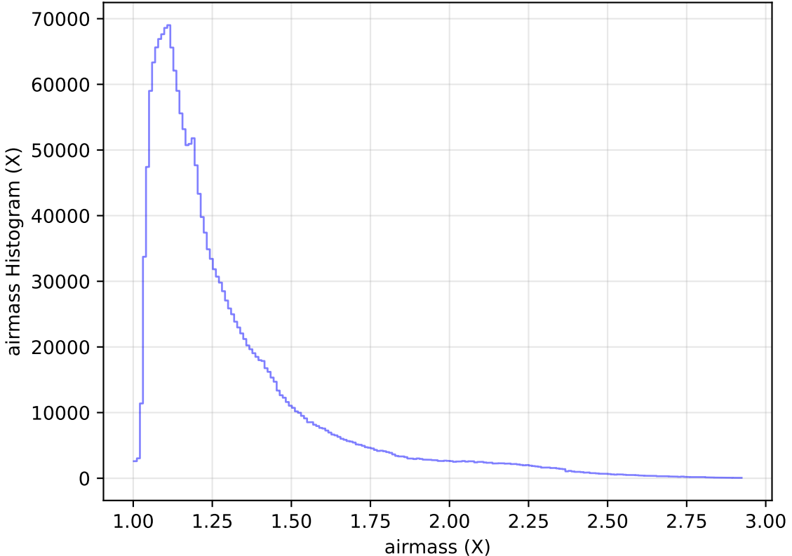
too_elab_heavy_r64_d3_ugrizy_v3.4_10yrs All sky all bands: airmass Histogram
