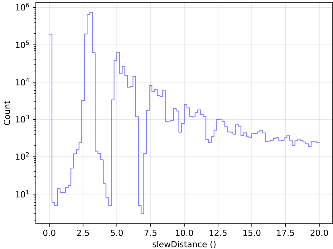
too_elab_heavy_r64_d3_ugrizy_v3.4_10yrs All visits: Zoom Slew Distance Histogram
