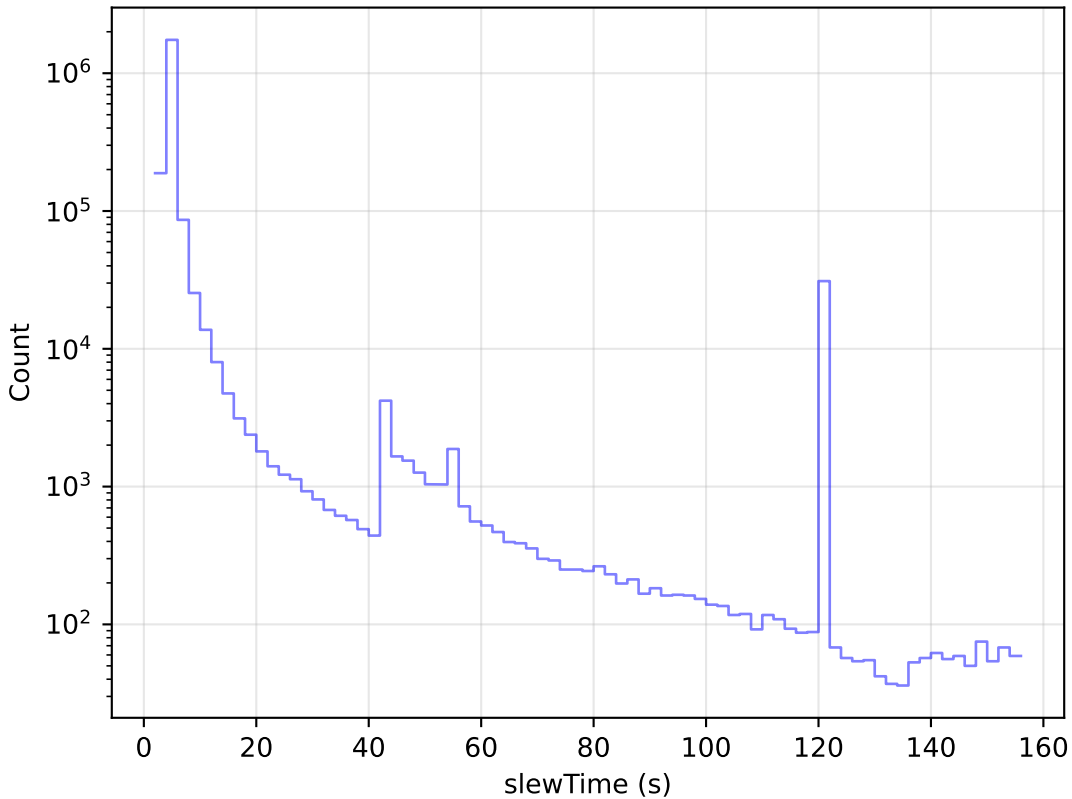
too_elab_heavy_r64_d3_ugrizy_v3.4_10yrs All visits: Slew Time Histogram
