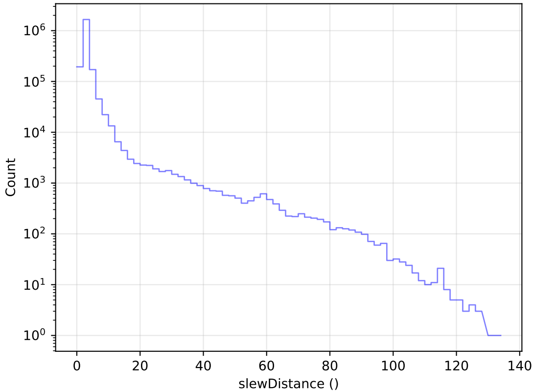
too_elab_heavy_r64_d3_ugrizy_v3.4_10yrs All visits: Slew Distance Histogram
