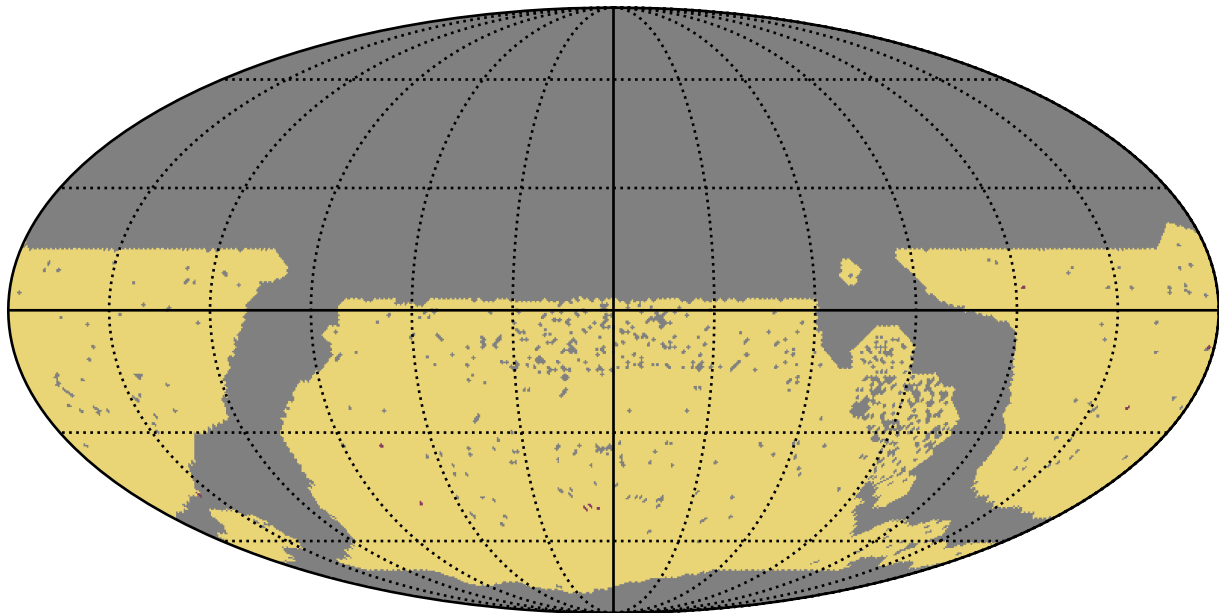
too_elab_heavy_r64_d3_ugrizy_v3.4_10yrs WFD: RapidRevisits
