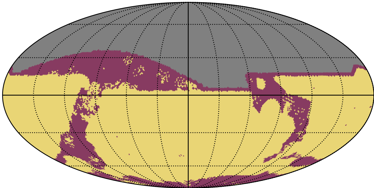
too_elab_heavy_r64_d3_ugrizy_v3.4_10yrs All sky: RapidRevisits
