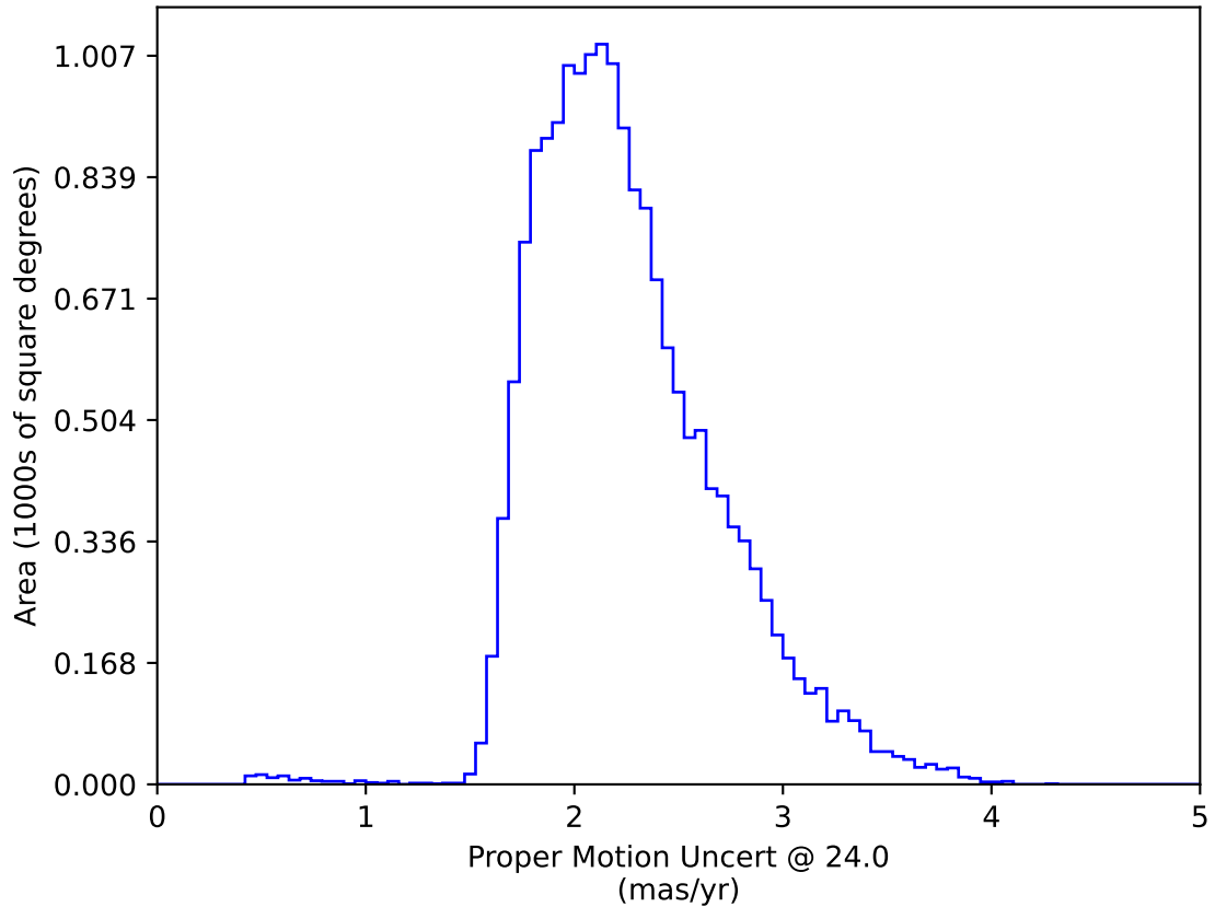
too_elab_heavy_r64_d3_ugrizy_v3.4_10yrs WFD: Proper Motion Uncert @ 24.0
