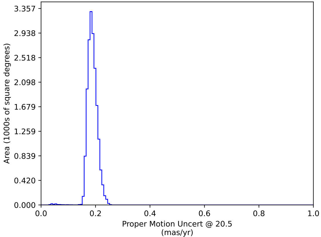
too_elab_heavy_r64_d3_ugrizy_v3.4_10yrs WFD: Proper Motion Uncert @ 20.5
