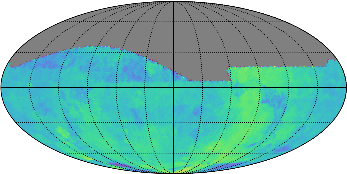
too_elab_heavy_r64_d3_ugrizy_v3.4_10yrs All sky: Parallax Coverage @ 24.0
