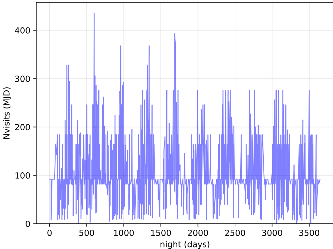
too_elab_heavy_r64_d3_ugrizy_v3.4_10yrs DDF: Nvisits
