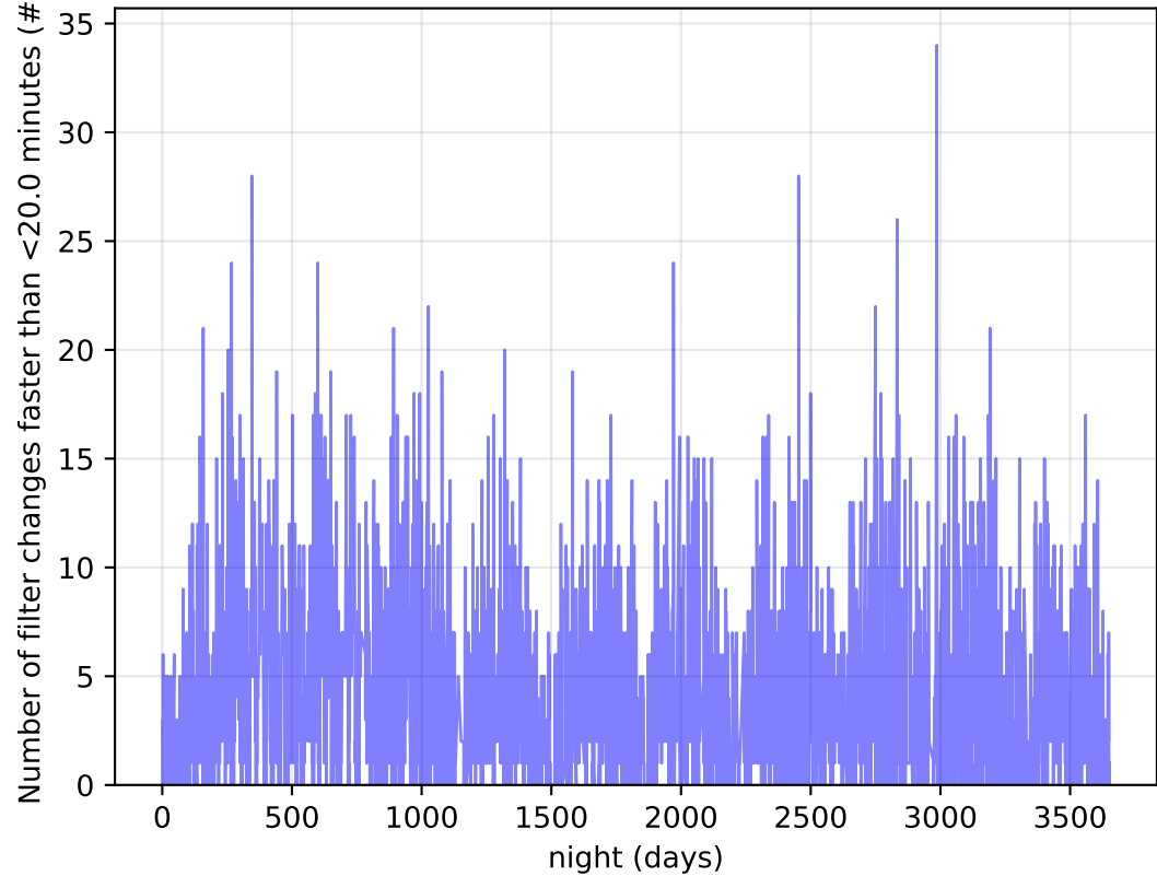
too_elab_heavy_r64_d3_ugrizy_v3.4_10yrs Per Night: Number of filter changes faster than <20.0 minutes
