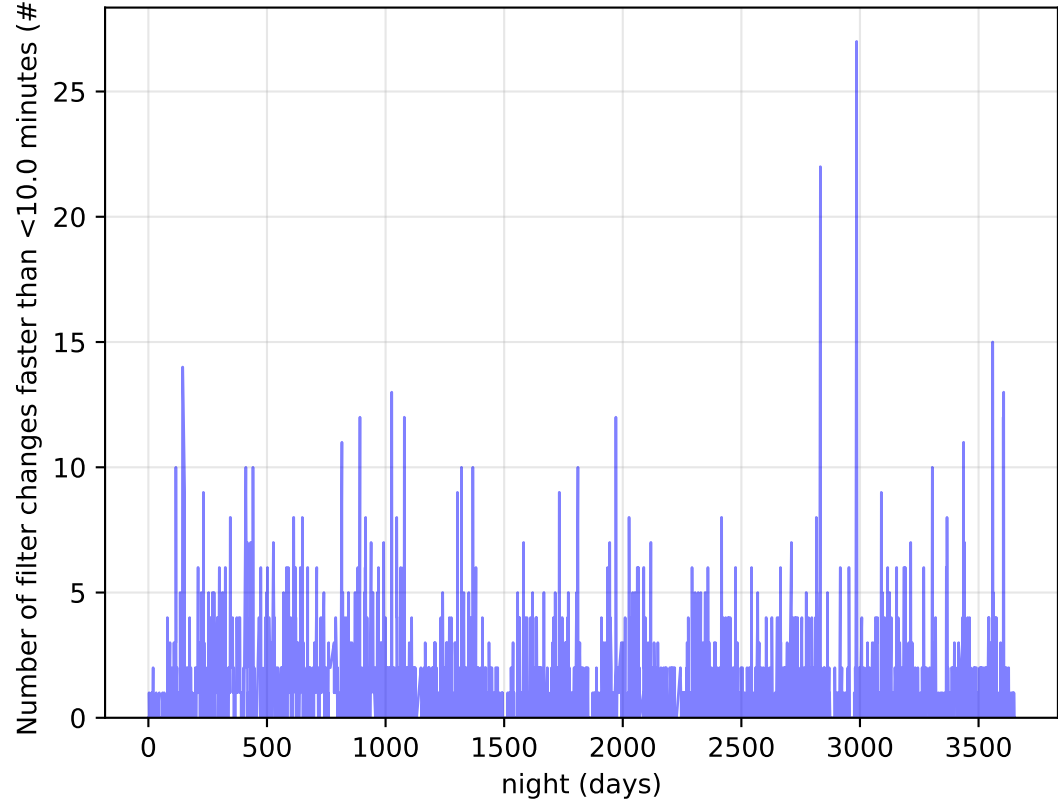
too_elab_heavy_r64_d3_ugrizy_v3.4_10yrs Per Night: Number of filter changes faster than <10.0 minutes
