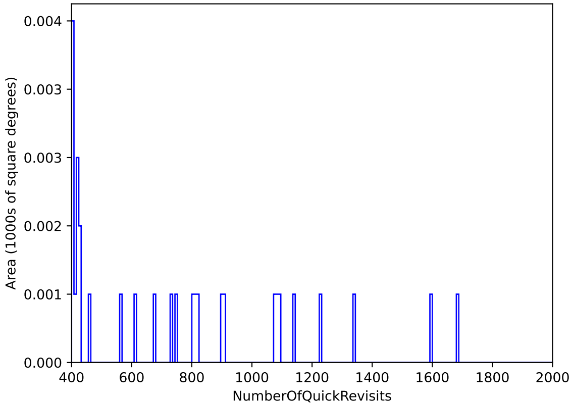
too_elab_heavy_r64_d3_ugrizy_v3.4_10yrs WFD: NumberOfQuickRevisits
