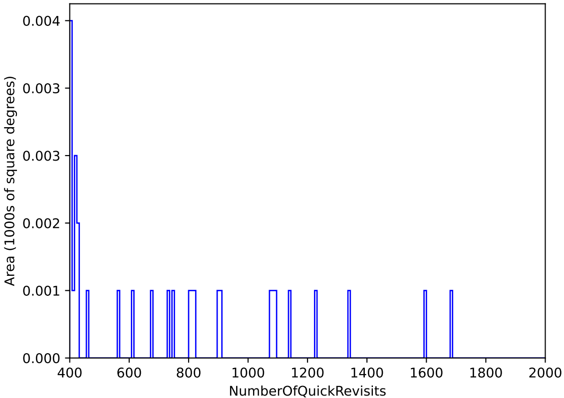
too_elab_heavy_r64_d3_ugrizy_v3.4_10yrs All sky: NumberOfQuickRevisits
