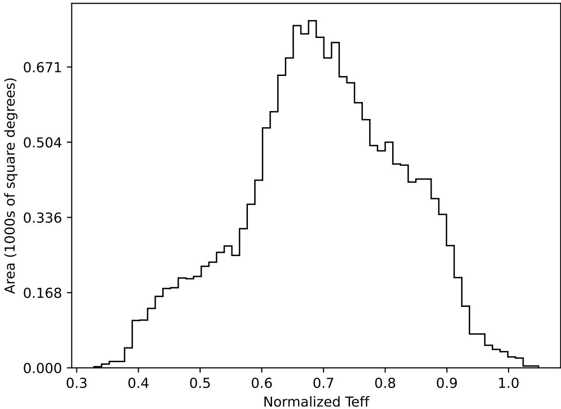
too_elab_heavy_r64_d3_ugrizy_v3.4_10yrs WFD all bands: Normalized Teff
