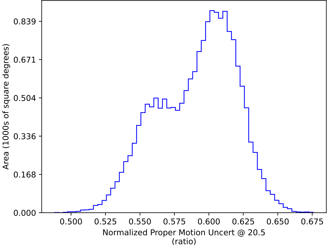
too_elab_heavy_r64_d3_ugrizy_v3.4_10yrs WFD: Normalized Proper Motion Uncert @ 20.5
