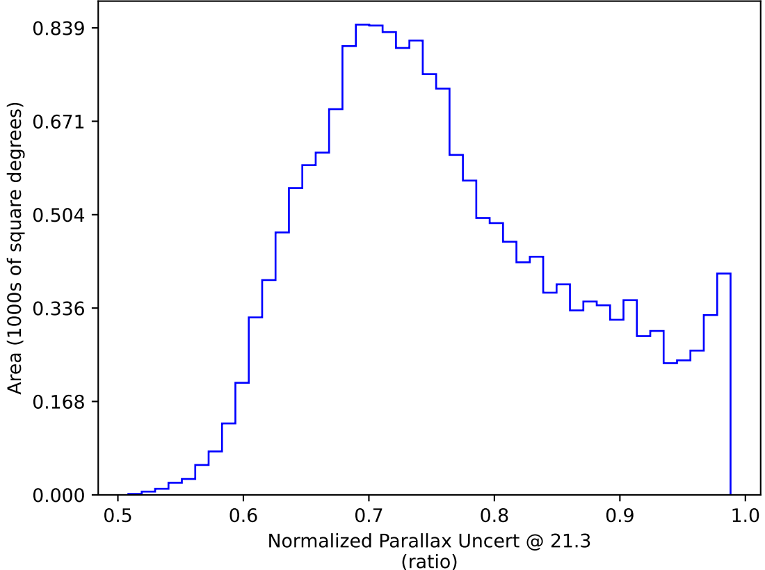
too_elab_heavy_r64_d3_ugrizy_v3.4_10yrs WFD y band only: Normalized Parallax Uncert @ 21.3
