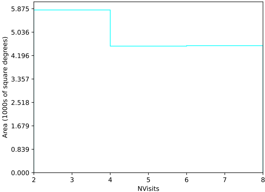
too_elab_heavy_r64_d3_ugrizy_v3.4_10yrs Yr 3-4 u band: NVisits
