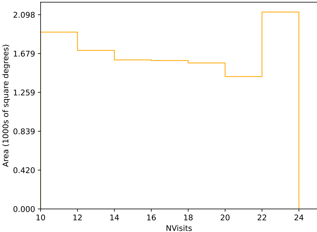
too_elab_heavy_r64_d3_ugrizy_v3.4_10yrs Yr 3-4 r band: NVisits
