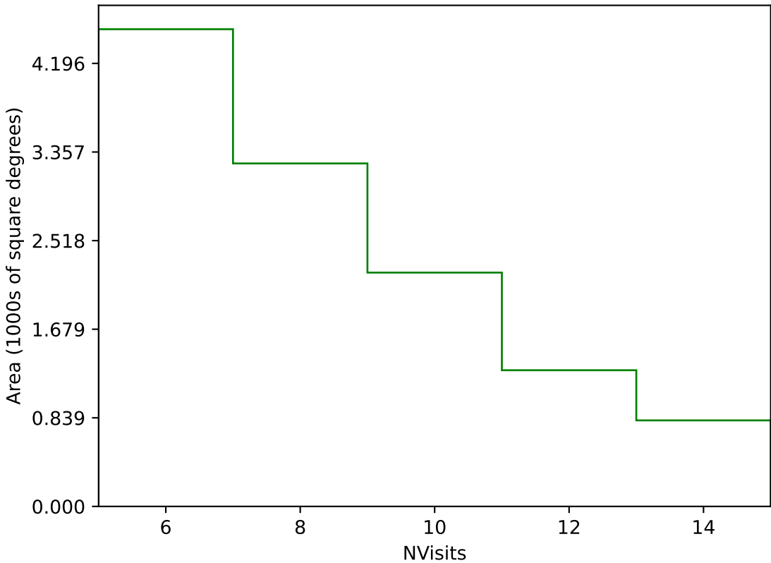
too_elab_heavy_r64_d3_ugrizy_v3.4_10yrs Yr 3-4 g band: NVisits
