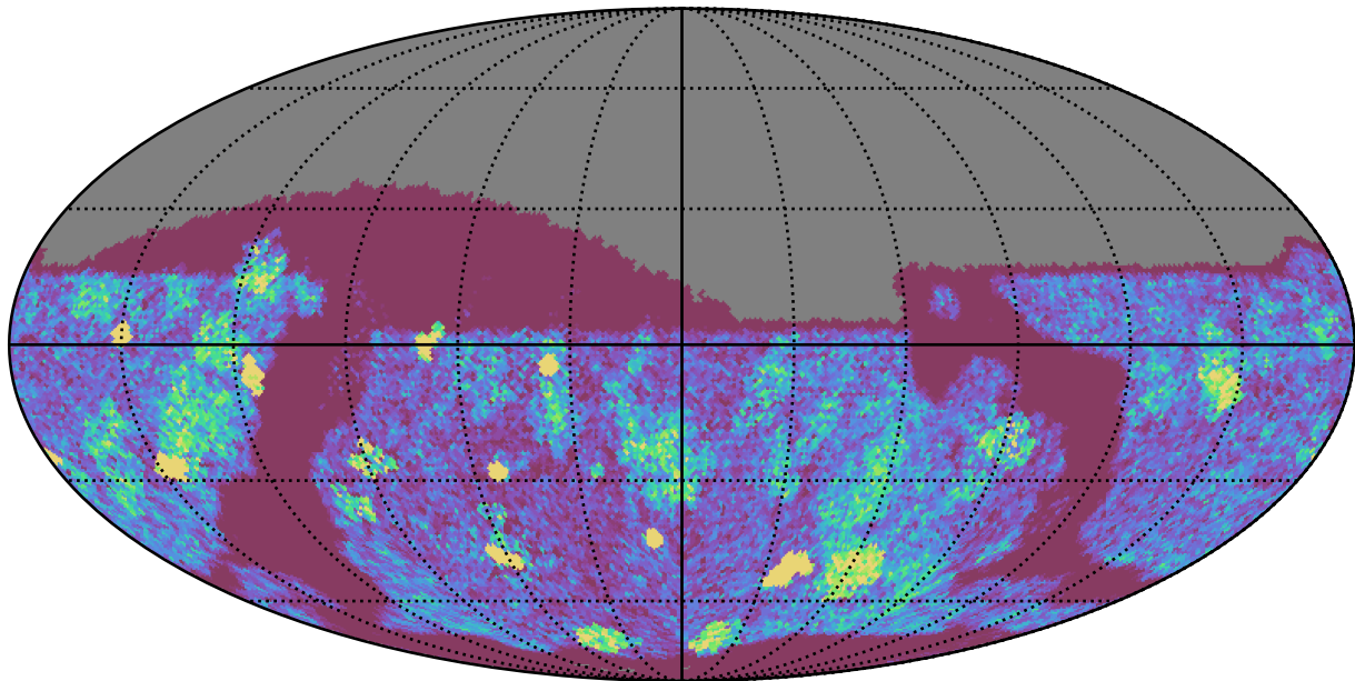
too_elab_heavy_r64_d3_ugrizy_v3.4_10yrs Yr 1 z band: NVisits
